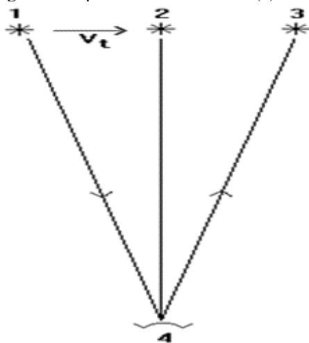
Fig.10: The past (1), verily (2) and the future (3) positions of astronomical object. Portion of light emitted by object in position (1) reaches observer (4) many years after. During this time the object that moves perpendicular to observer with speed v_t , moves to position (2). If at the moment of record portion of light were emitted for point of observation it would meet object in point (3).
