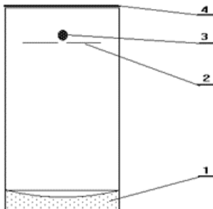
Fig.9: Scheme of Kozyrev telescope. 1 – focusing mirror, 2 - slot, 3 - detector, 4 – light-proof lid.
