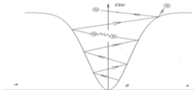
Fig.11: Oscillation of Nitrogen molecule in potential well of catalyst.
