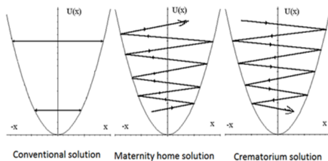
Fig. 8: Solution of UQT for harmonic oscillator.
