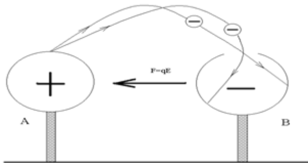
Fig. 7: Work for transferring the charge depends on the mode of transferring and on the path.
