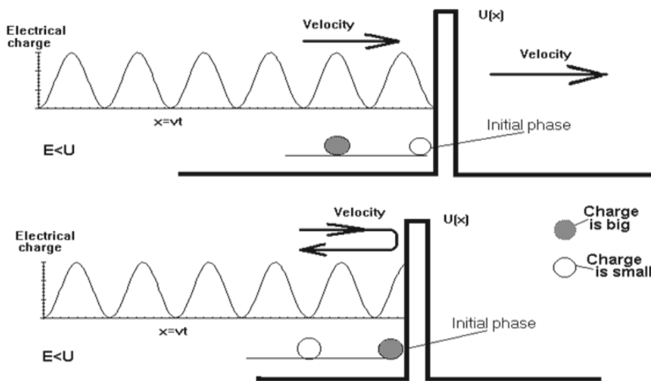
Fig.12: Illustration of the tunnel effect.
