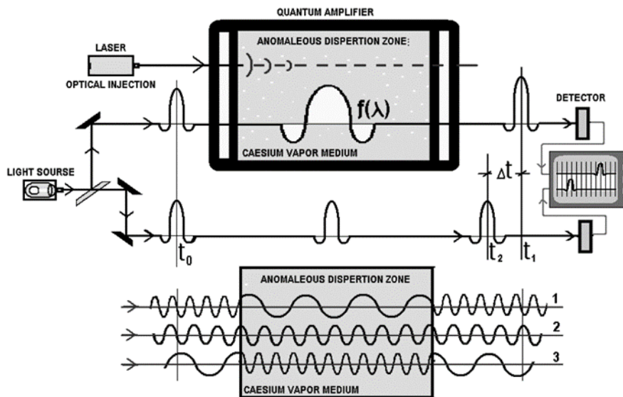
Fig. 5: Experiments of L.Wang - superluminal light propagation.
