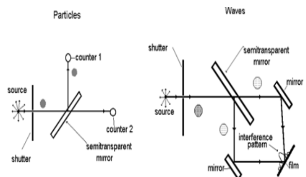
Fig.1: Experiments with individual photons on semitransparent mirror
