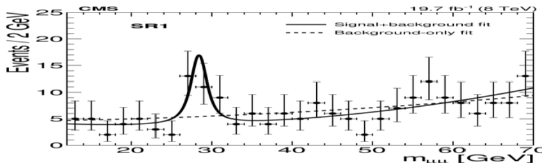
Fig.6: Peak of energy at 28GeV.
