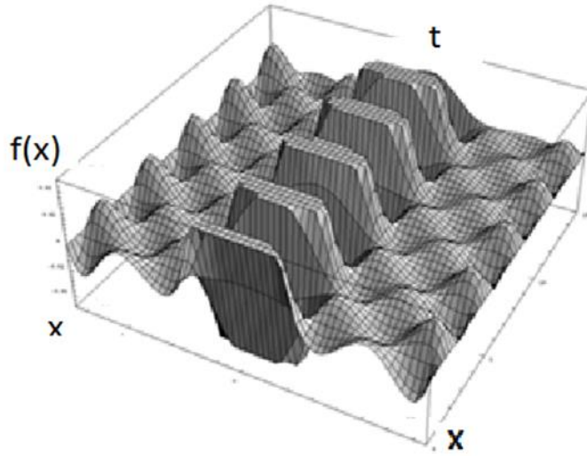
Fig. 2: During the motion, the packet f(x) will appear and disappear periodically.
