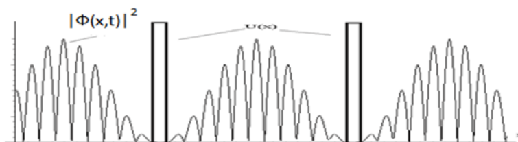
Fig.13: Visual image of particles passing through two potential barriers - scheme of New Maxwell Demon.
