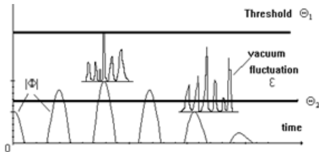
Fig.4. Quantum measurements.
