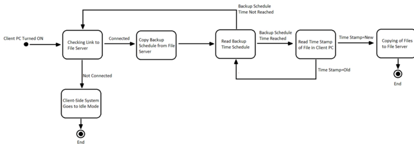
Fig 3: State Transition Diagram.
