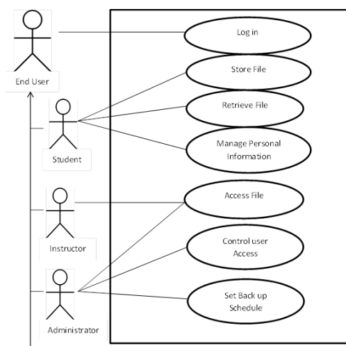
Fig 1: Use Case Diagram of the System.
